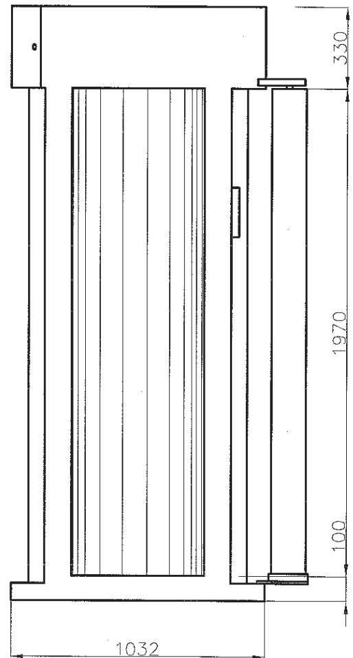
VISTA LATERALE SIDE VIEW
